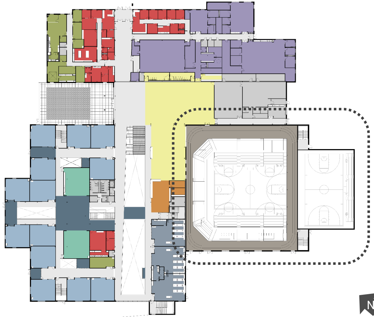
Floor Plan – Level 01
